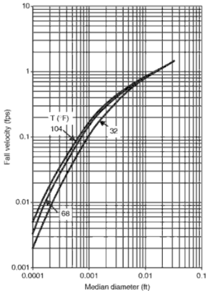
Figure 10.4-4. Particle fall velocity (Ref. 10-35).
