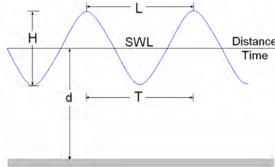
Figure 10.2-10. Wave Parameters.
